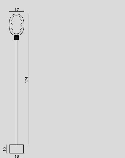
LU1615.1L PIANTANA / FLOOR LAMP with dimmer push button Glass Ø 17 cm - H 174 cm 1 x LED 9W DIMM - 350 mA - 2700 or 3000°K
